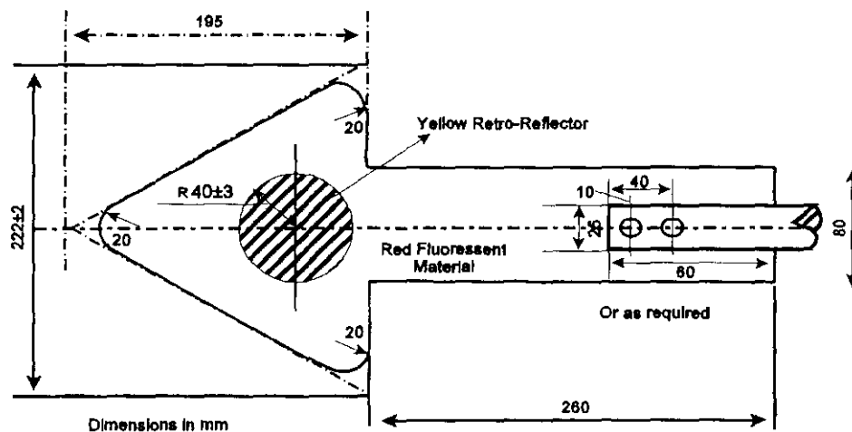
PORTABLE DIRECTION INDICATOR
